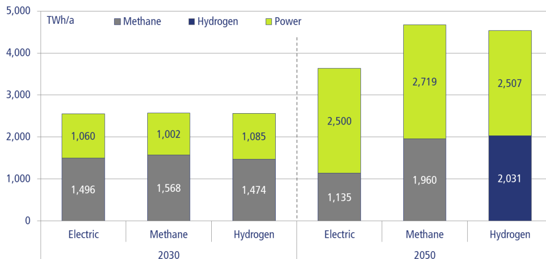
Figure 4-12 Cross-border energy transport within EU28
