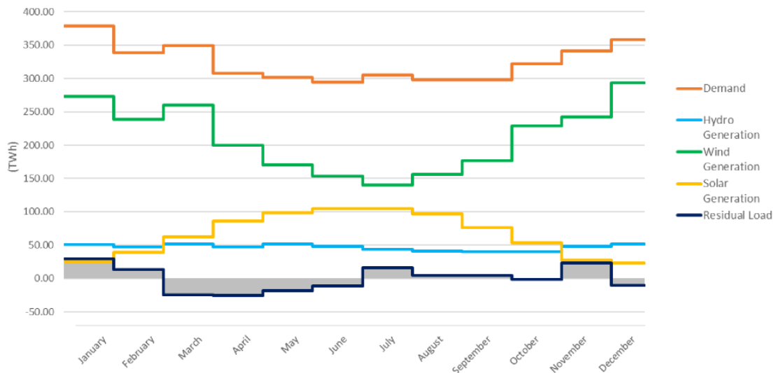
Figure 5 – 100% RES 2040 scenario
